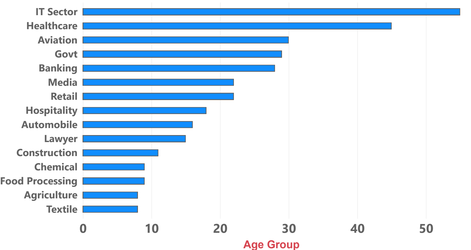
Age Group by Occupation
